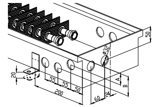
KORAFLEX FV 9/28 A=50, B=60
